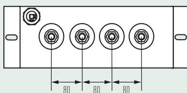
4 terminals_4 Anschlüsse
