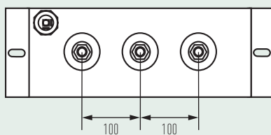
3 terminals_3 Anschlüsse
